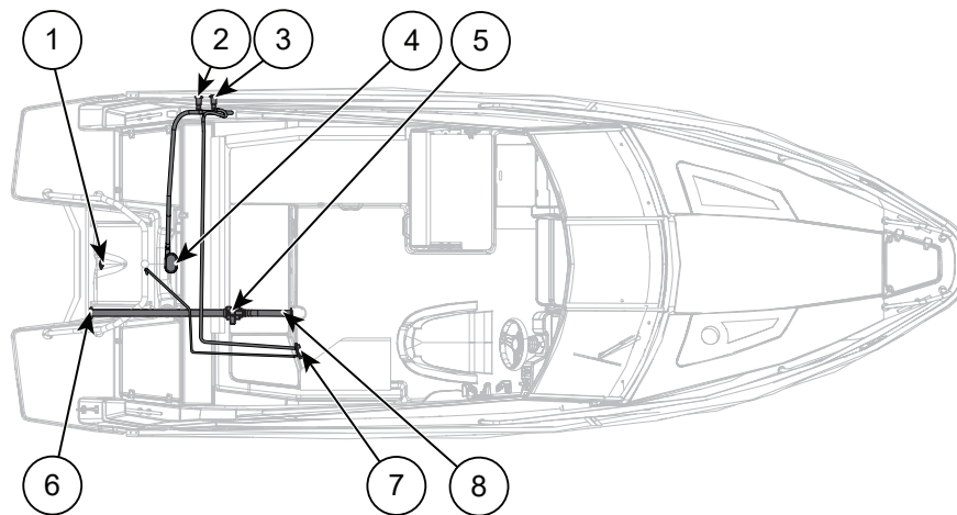
Figure 9.1 Yamarin 63 DC bilge pumps and draining
