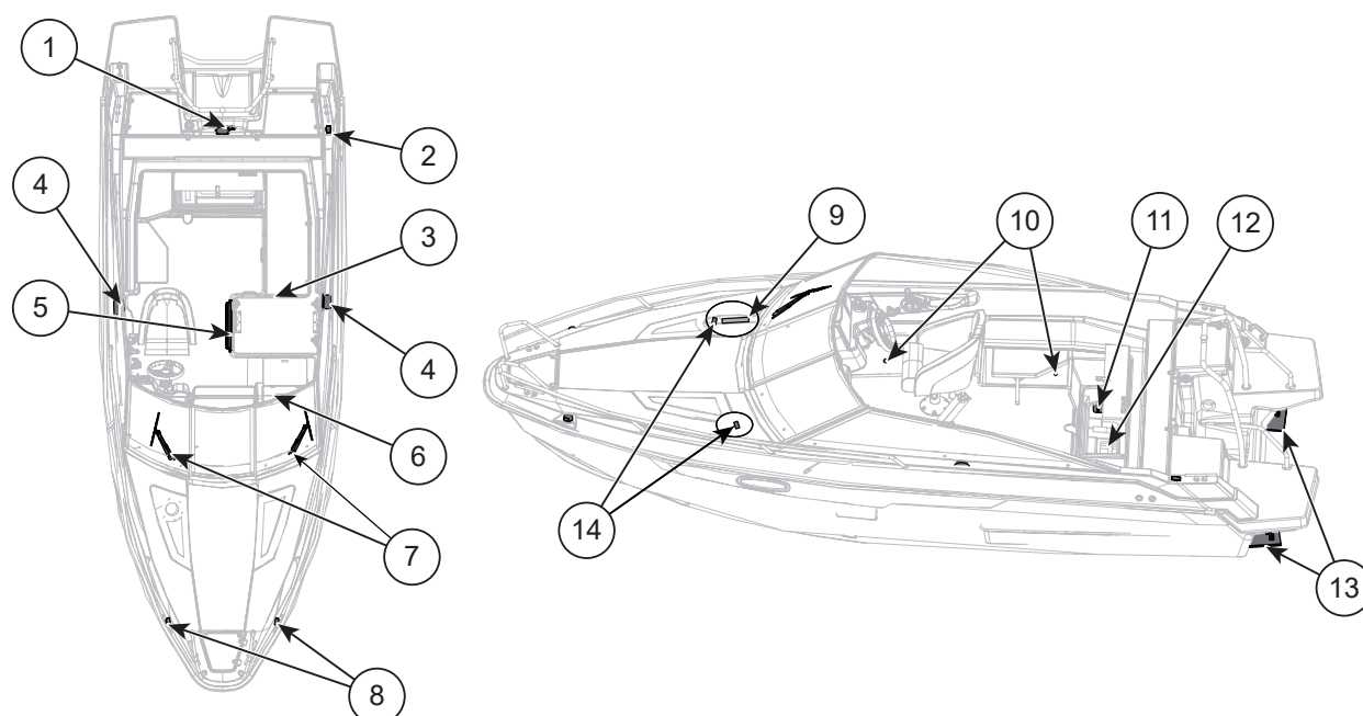
Figure 8.4 Yamarin 63 DC electrical equipment
