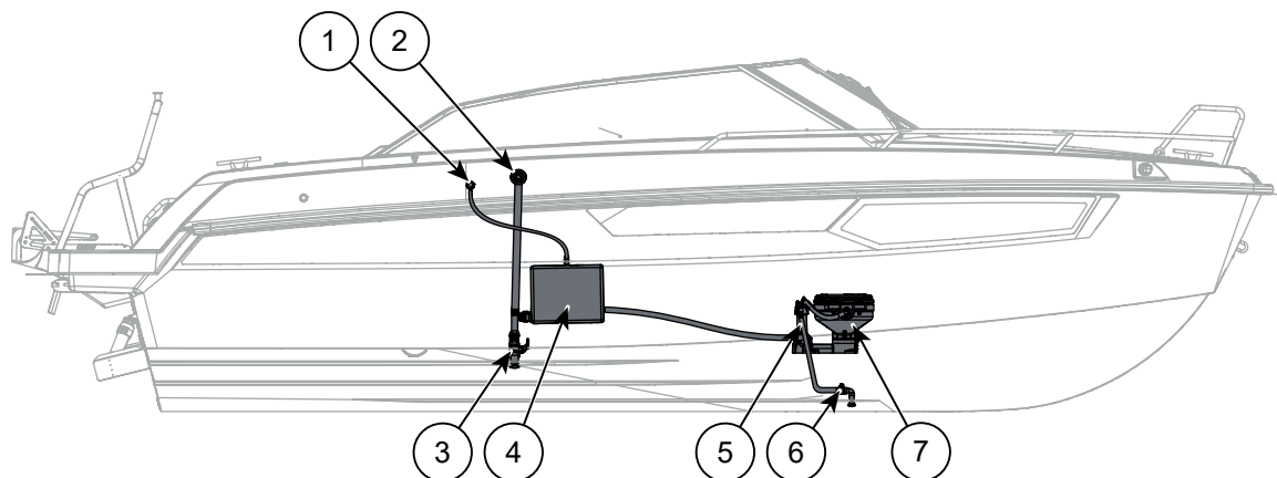
Figure 11.1 Yamarin 67 DC septic system
